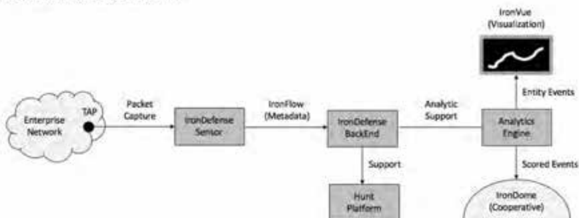
Figure 4-1. IronDefense Processing Flow
